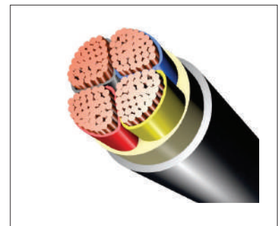
LOW VOLTAGE POWER CABLE MULTICORE
